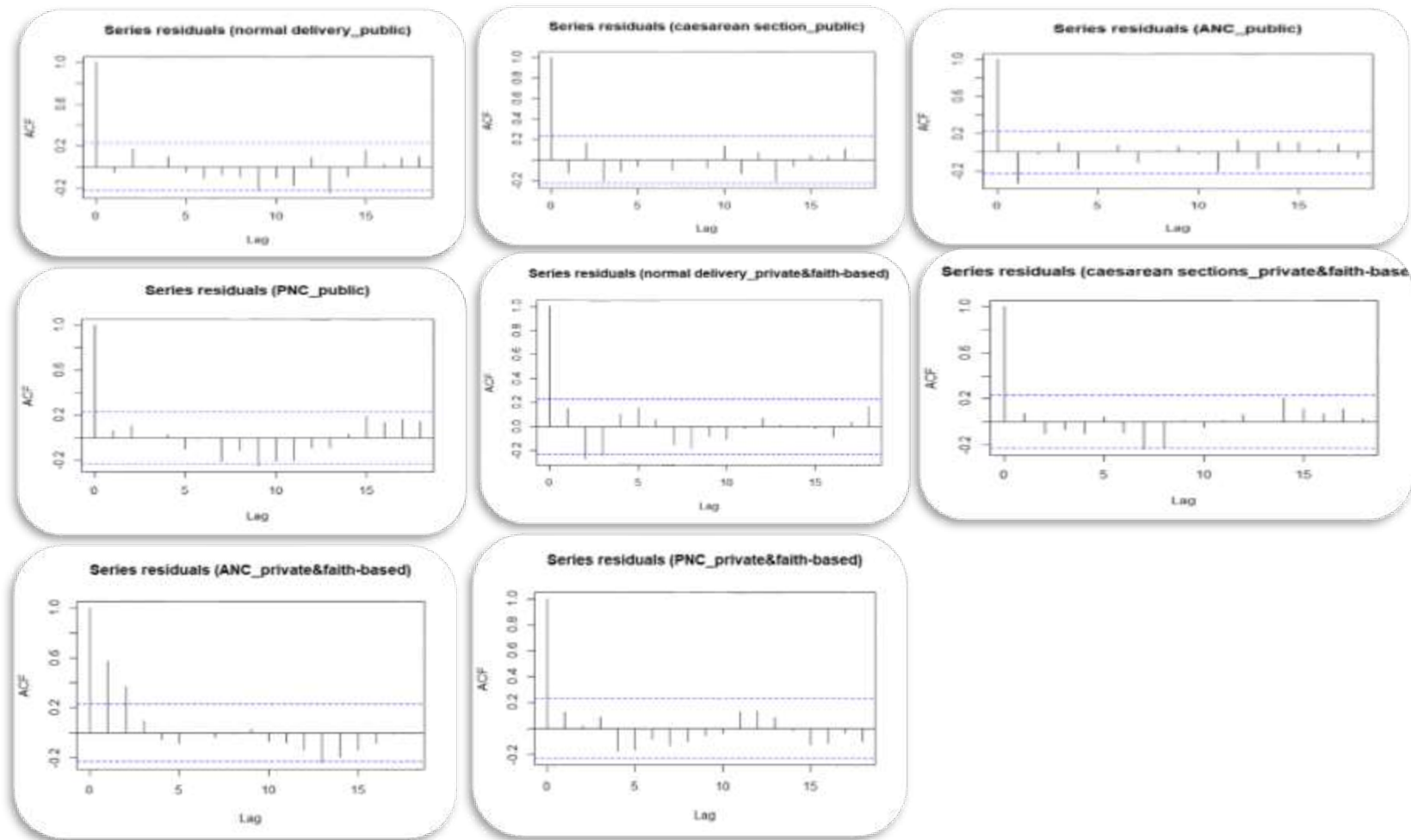
Supplementary Figure 3: Autocorrelation function (ACF) plots for the ITS in public, private and faith-based facilities
